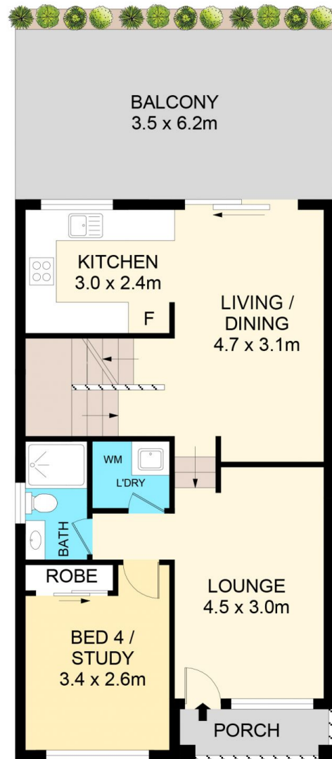
GROUND LEVEL
